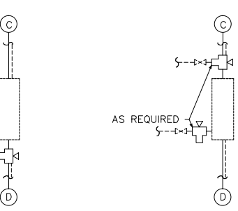
GAUGE GLASS AND MAGNETIC INDICATOR CONNECTIONS
