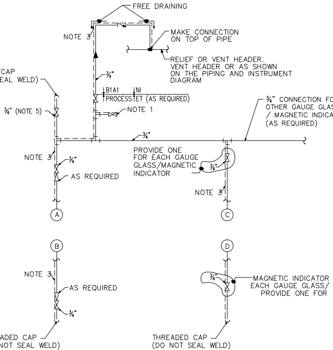
DETAIL OF STP DWG 8-140-7
