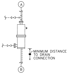
EXTERNAL DISPLACEMENT LEVEL INSTRUMENT CONNECTIONS
