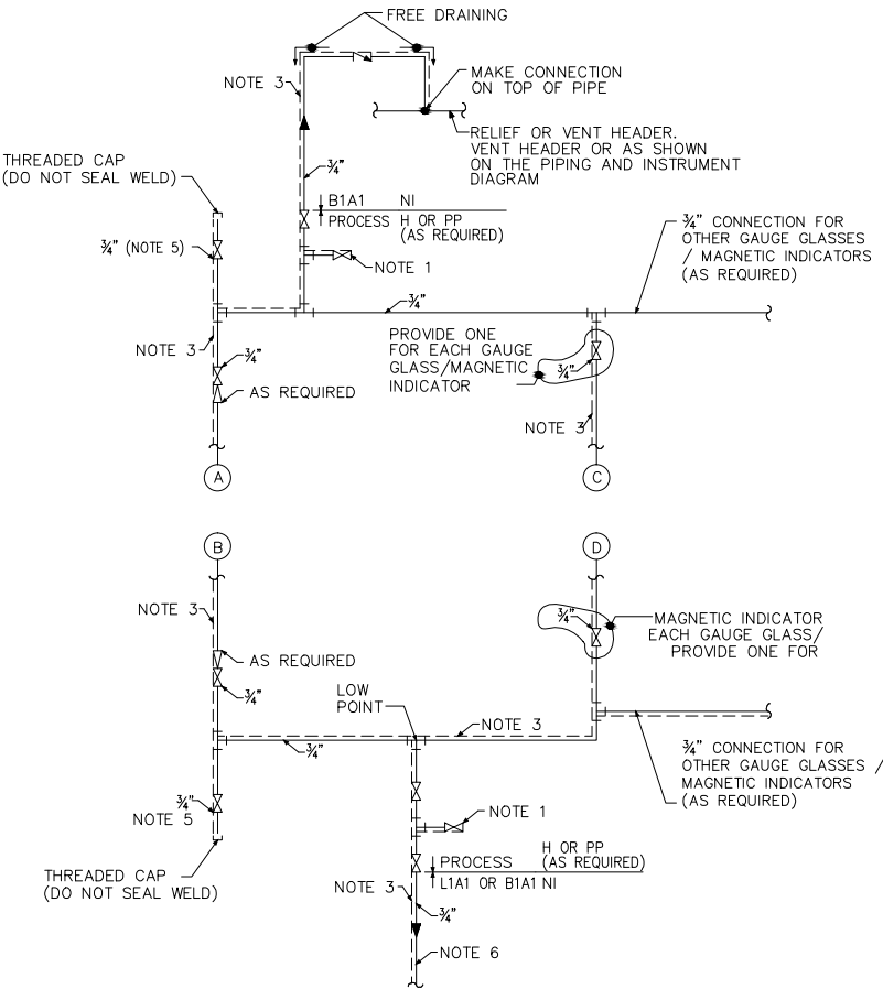
DETAIL OF STP DWG 8-139-8
